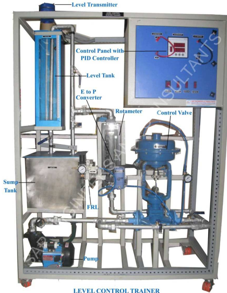
LEVEL CONTROL TRAINER
